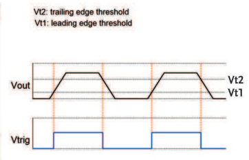
Vtrig Timing Chart
